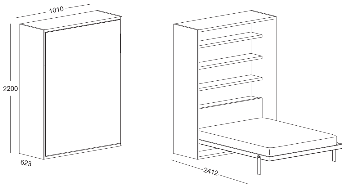
Details of the patented bed base CF09
